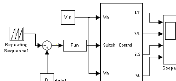
Fig. 9(b) Subsystem for Cuk converters
