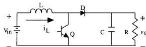
Fig. 3 DC-DC Boost Converter
